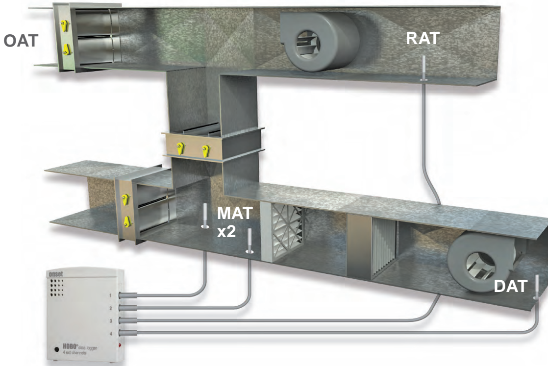
Four-channel logger deployment for ventilation air control verification
