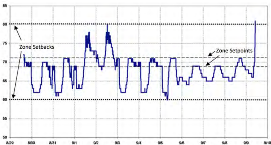
Figure 4: Proper Function of Zone Temperature Setpoints and Setbacks
