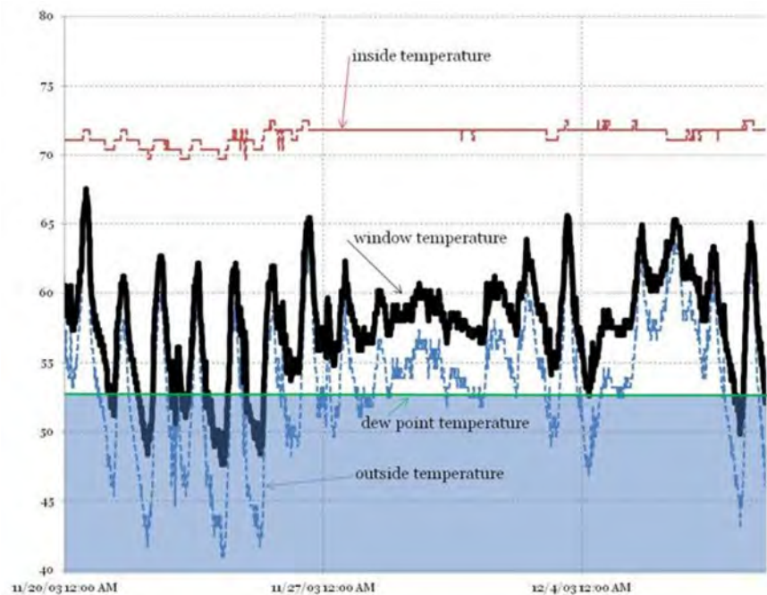
Figure 9: Moisture Investigation
