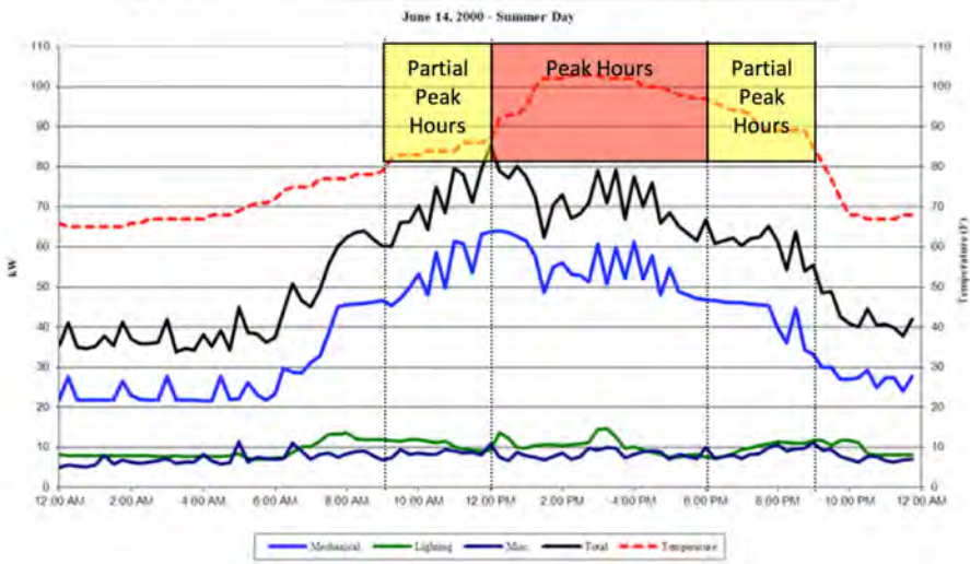
Figure 12: Peak Loads Occur During Utility Peak Demand Periods
