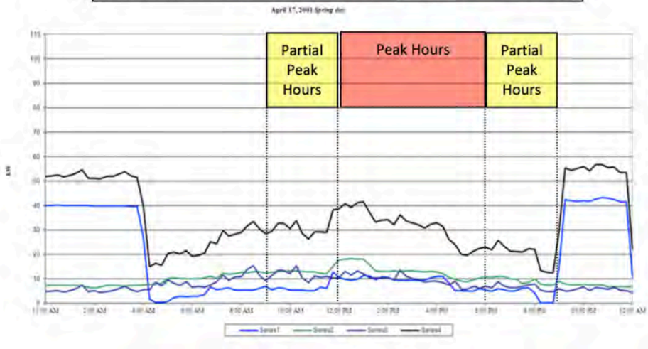
Figure 13: Peak Loads Shifted Out of Utility Peak Demand Periods
