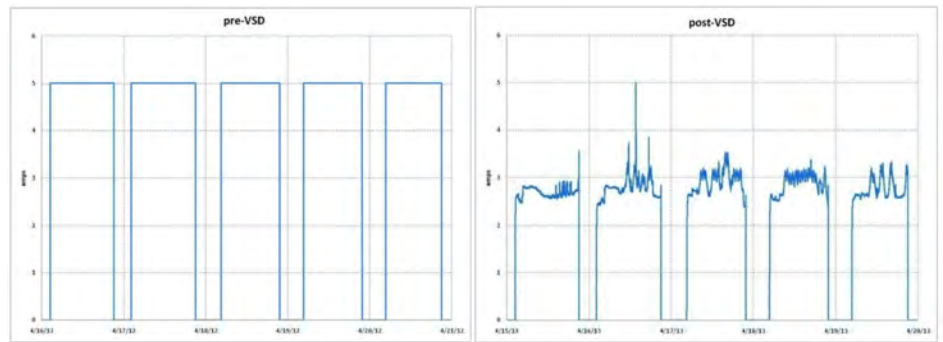
Figure 11: Pre- and Post-Implementation of Variable Speed Drive
